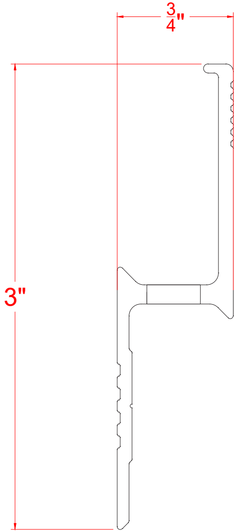
X-Z19PF PROFILE
