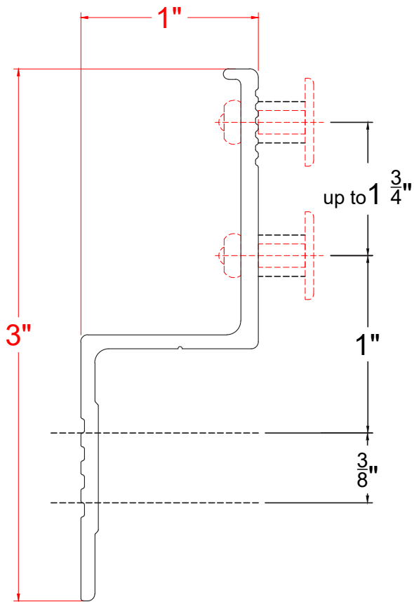
X-Z25 PROFILE
